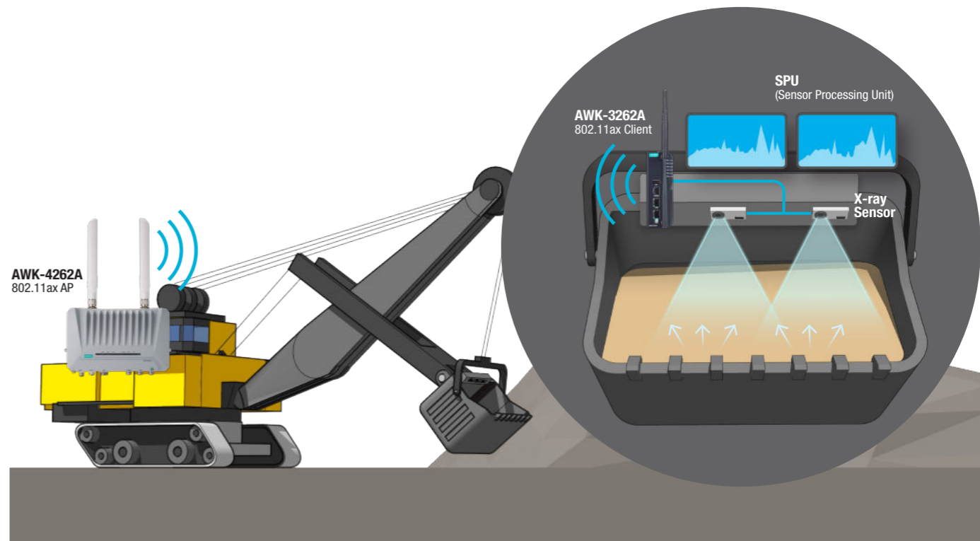
AWK-3262A 802.11ax Wireless AP/Client
